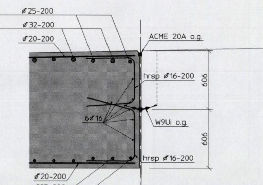
Detail 2
