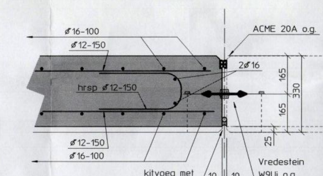
Detail 5
