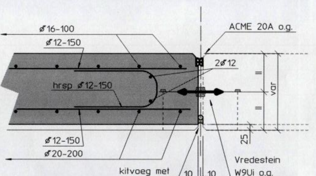
Detail 3
