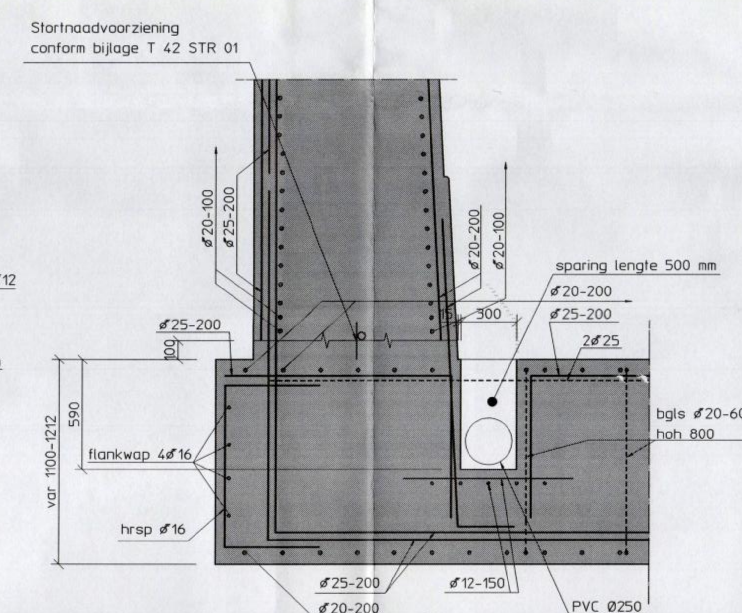
Detail 6
