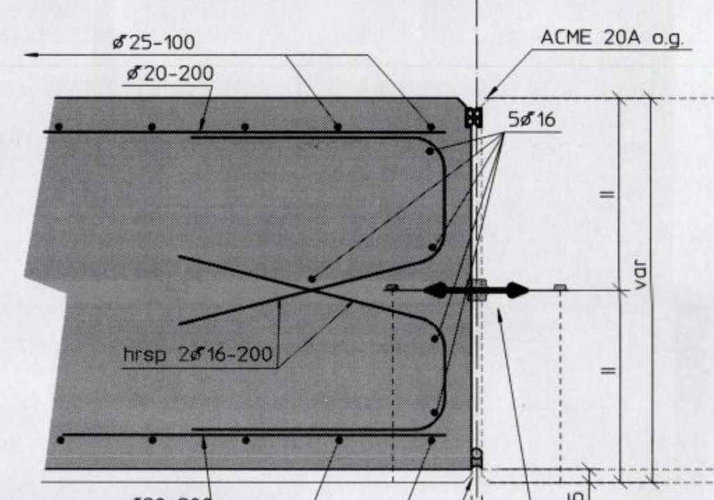
Detail 4
